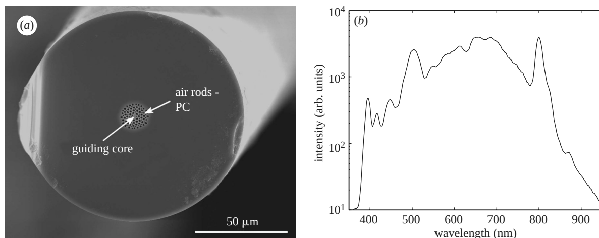
Figure 9. (a) SEM cross-sectional view of silica photonic crystal fibre without external cladding (reproduced courtesy of W. Belardi, ORC, University of Southampton). (b) Spectrum of supercontinuum obtained from PCF.
