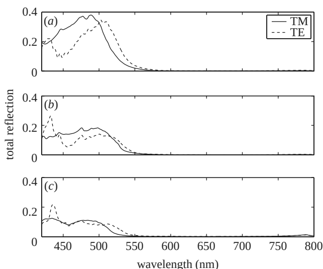
Figure 12. Total reflection of M. rhetenor microstructure for angles of incidence of (a) 10°, (b) 30° and (c) 60°, and both polarizations.
