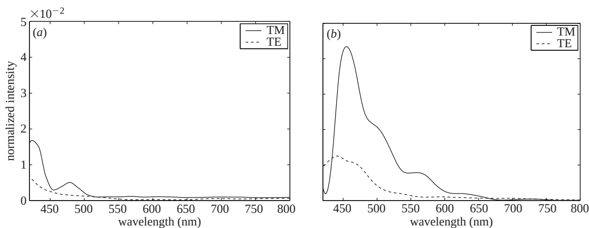
Figure 8. Computed diffraction efficiencies of model (ii) for a 30^\circ angle of incidence and both polarizations. Graph of the (a) zeroth order of diffraction (specular reflection) and of (b) the first order of diffraction.
