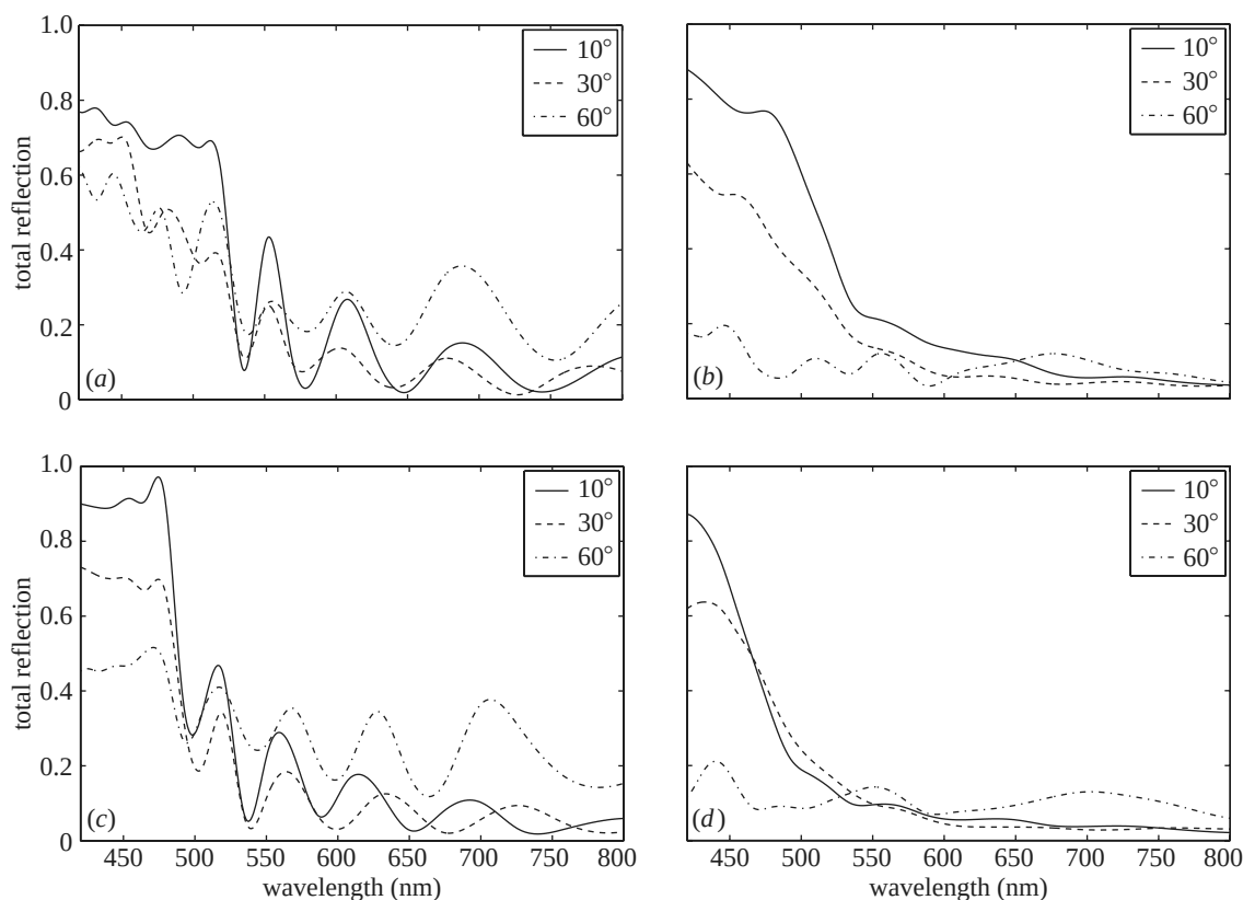
Figure 7. Computed spectra of the total reflection for TE polarization and angles of incidence in models (i)–(iv). The lettering corresponds to that of figure 4.
